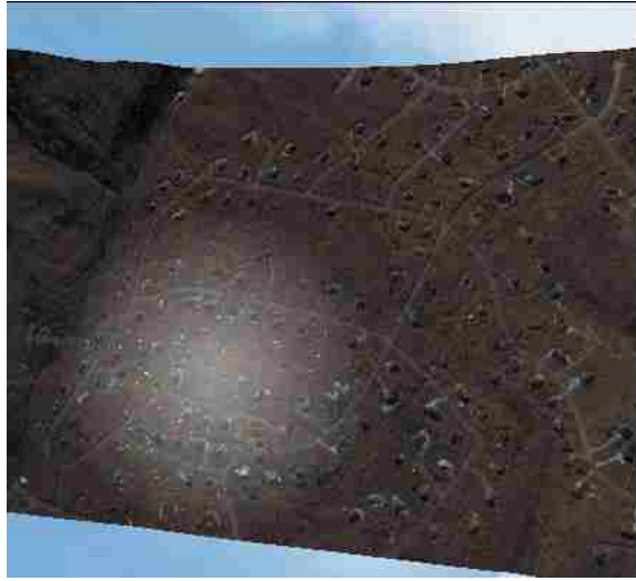
Figure 5.4: Gaussian distribution
